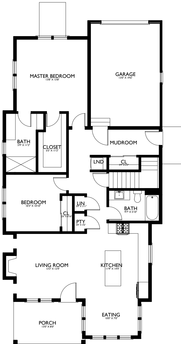
FLOOR PLAN 1265 SQ FT
